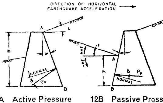
FIG. 12 EARTH PRESSURE DUE TO EARTHQUAKE ON RETAINING WALLS
