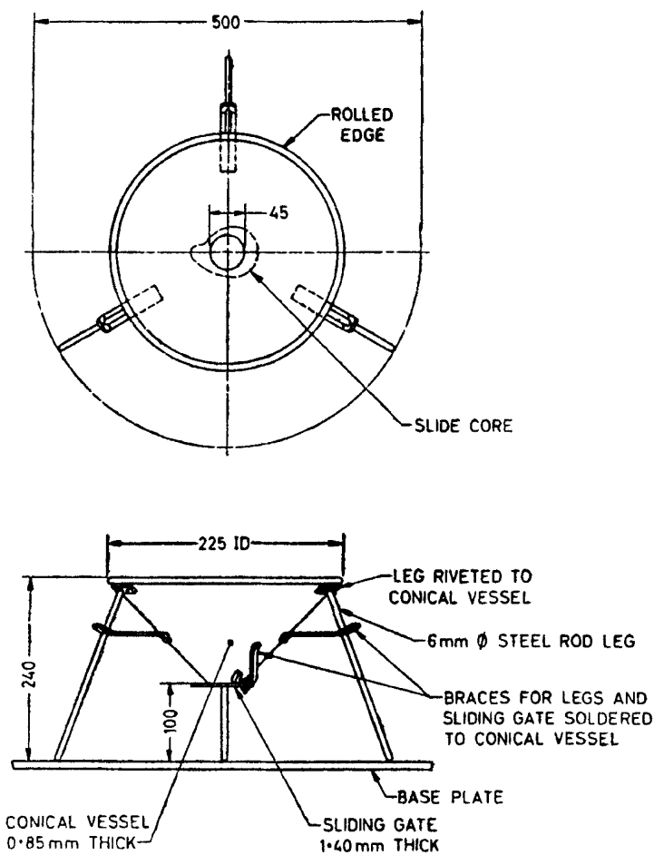
FIG. 1 CONSISTOMETER
